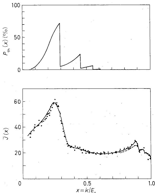
Fig. 5a. - Photon intensity and polarization from diamond target; experimental spectra compared with the averaged intensity and theoretical polarization for \alpha = 89^\circ , \theta = 50 mrad, E_0 = 4.8 GeV. — Hartree potential, --- exponential potential.
