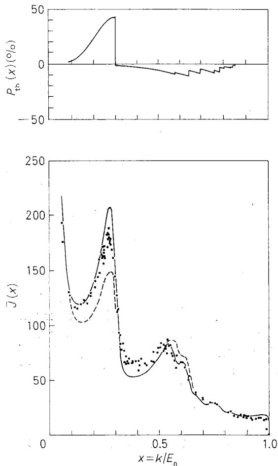
Fig. 2a. - Photon intensity and polarization from diamond target; experimental spectra compared with the averaged intensity and theoretical polarization for \alpha = 0^\circ , \theta = 3.44 mrad, E_0 = 4.8 GeV. — Hartree potential, --- exponential potential.
