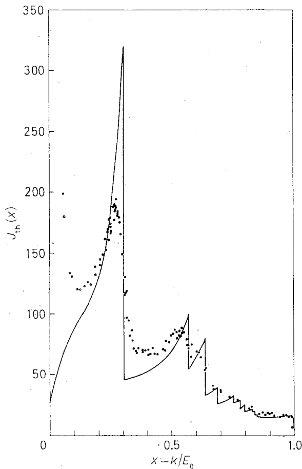
Fig. 2. - Photon intensity from diamond target; experimental spectra compared with the theoretical intensity I_{th} (full line) for \alpha = 0^\circ , \theta = 3.44 mrad, E_0 = 4.8 GeV \Delta\theta = \Delta\alpha = 0 .
