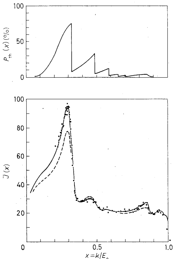
Fig. 4a. - Photon intensity and polarization from diamond target; experimental spectra compared with the averaged intensity and theoretical polarization for \alpha = 1.5^\circ , \theta = 50 mrad, E_0 = 4.8 GeV. — Hartree potential, --- exponential potential.
