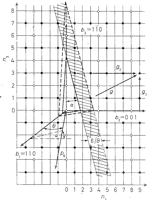
Fig. 1. — Orientation of electron momentum P_0 in the reciprocal lattice space of the diamond, schematic.
