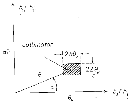
Fig. 6. - Relation between \theta, \alpha and \theta_H, \theta_V ; and area defined by collimation on the unit sphere, schematic.
