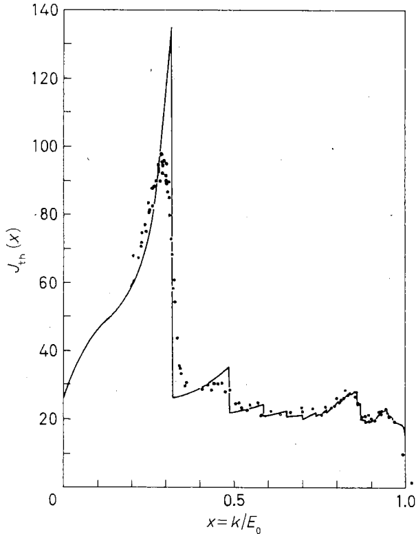
Fig. 4. - Photon intensity from diamond target; experimental spectra compared with the theoretical intensity I_{th} (full line) for \alpha = 1.5^\circ , \theta = 50 mrad, E_0 = 4.8 GeV,
