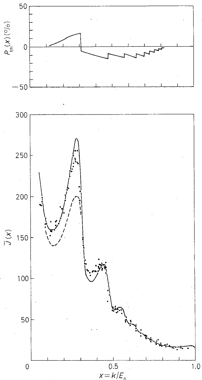
Fig. 3a. - Photon intensity and polarization from diamond target; experimental spectra compared with the averaged intensity and theoretical polarization for \alpha = 90^\circ , \theta = 2.48 mrad, E_0 = 4.8 GeV. — Hartree potential, --- exponential potential.
