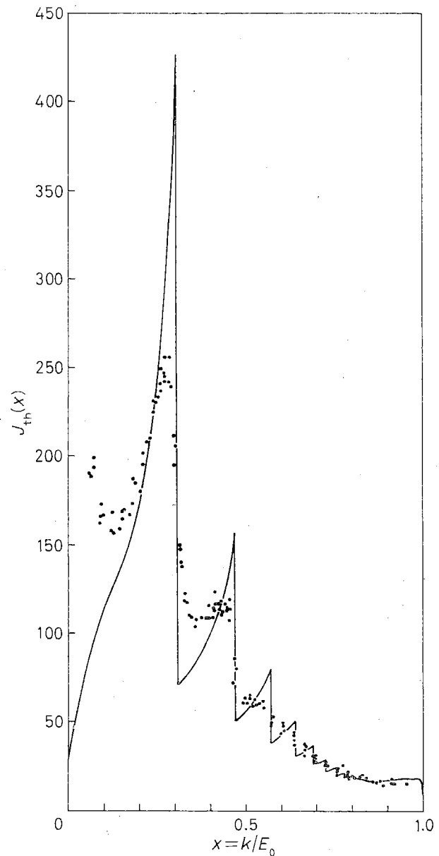
Fig. 3. - Photon intensity from diamond target; experimental spectra compared with the theoretical intensity I_{th} (full line) for \alpha = 90^\circ , \theta = 2.48 mrad, E_0 = 4.8 GeV, \Delta\theta = \Delta\alpha = 0 .
